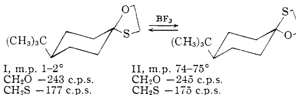
Fig. 1.—4- t -Butylcyclohexanone ethylene hemithioketals.
